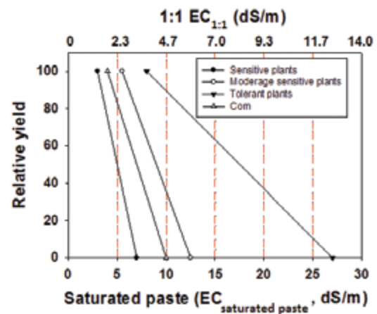
Figure 32.4 The relationships between the EC values measured multiple ways and relative yield. The conversion of EC 1:1 to EC saturate paste was based on Figure 32.3. Note: The values of dS/m are identical to mmhos/cm. (Courtesy of SDSU)
